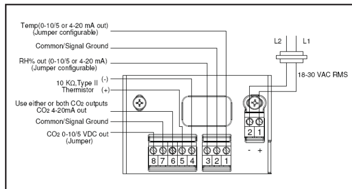
Figure 2: Display Unit Wiring for 4-Wire System, AC Power
