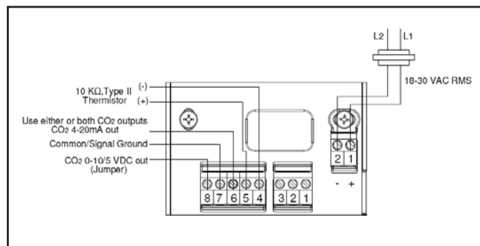
Figure 4: Non-Display Unit Wiring for 4-Wire System, AC Power
