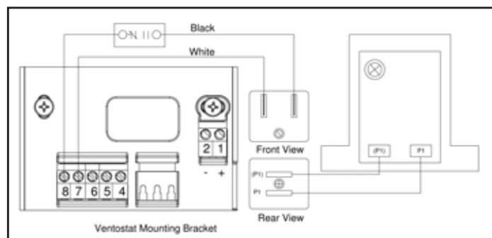
Figure 5: Wiring CO 2 Sensor Voltage Output to Honeywell M7415 Damper Actuator with W7459 Logic Module
