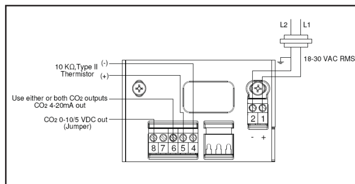
Figure 3: Non-Display Unit Wiring for 3-Wire System, AC Power
